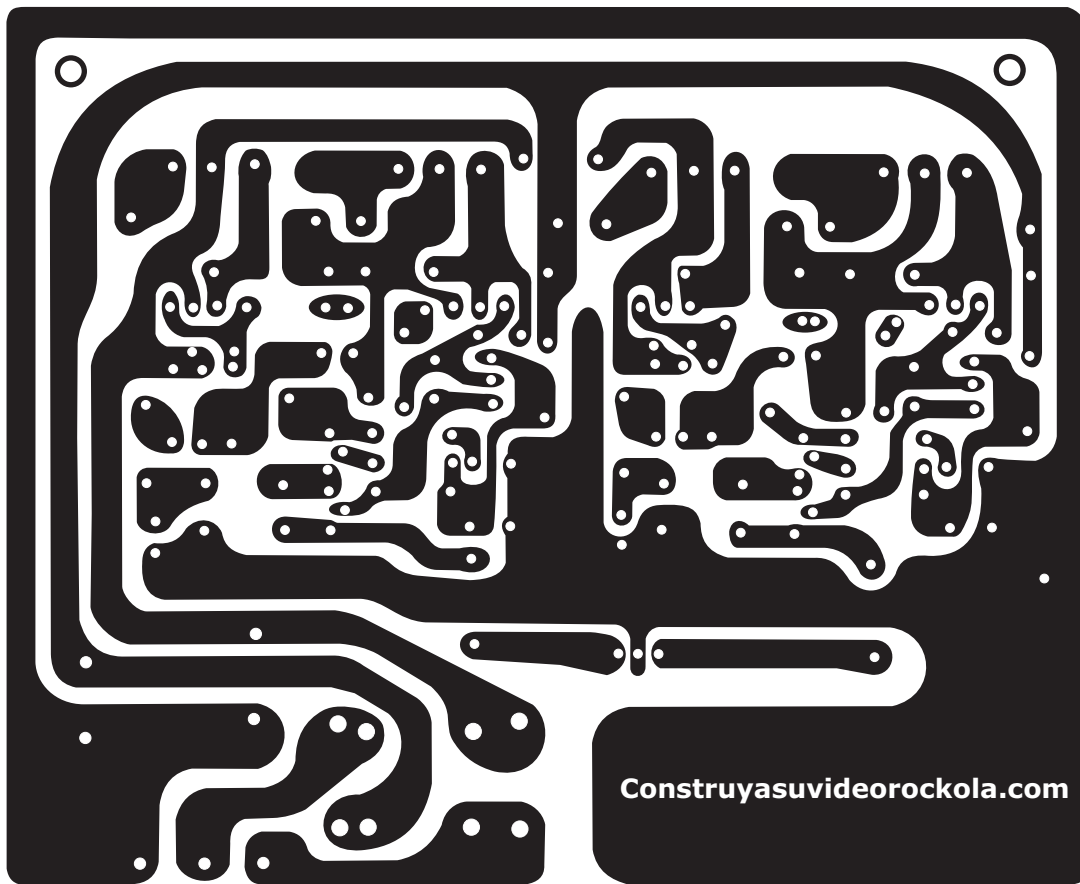
PCB
